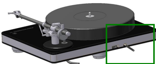
Pic. 10: Speed fine adjustment
